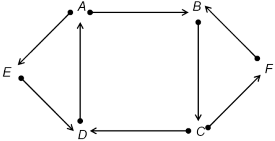
Diagram of possible allocation. An arrow between i and j represents d_{i,j} = 100
